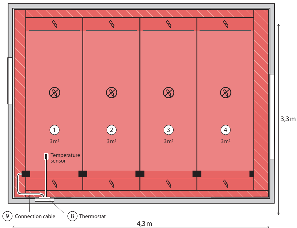
Fig. 19. Connectors along bottom wall and place for thermostat installation is bottom-left corner of the room.
