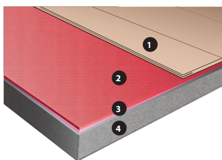
Fig. 16. Floor heating with DEVIDry™ on existing concrete subfloor
