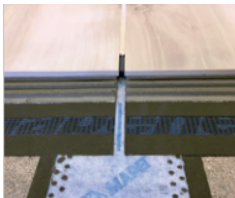
Mapeband Easy applied around a control joint in the screed
